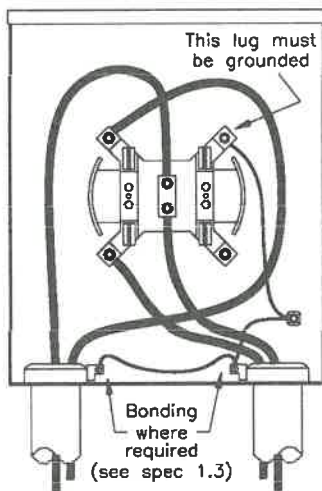
200a, 120v, 1ph, 2w
