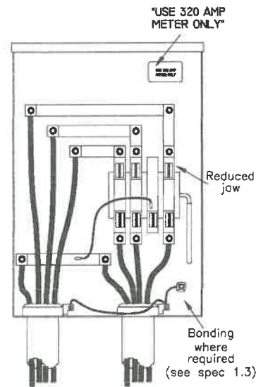
320/400a, 120/208v, 3ph, 4w
