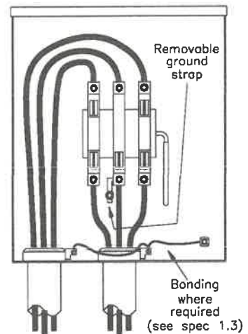
200a, 240v, 3ph, 3w
