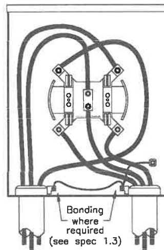
200a, 120/240v, 1ph, 3w
