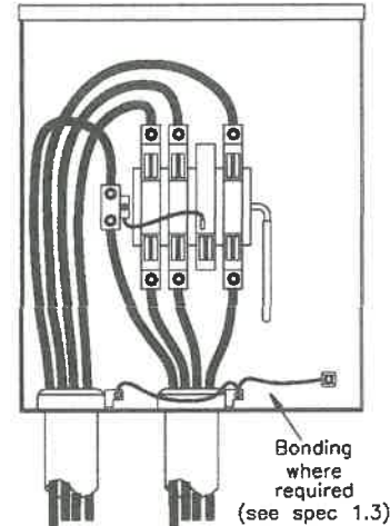
200a, 120/208v, 3ph, 4w
